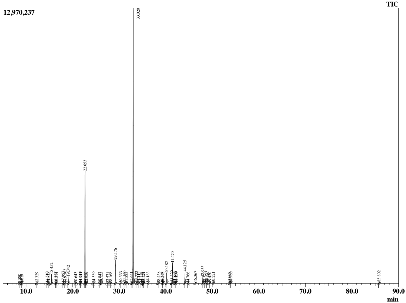
Chromatogram SalSci2
